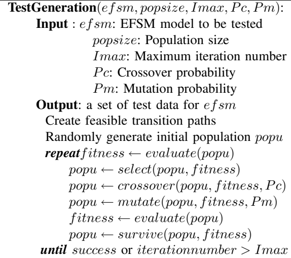
Figure 2. Test data generation algorithm
