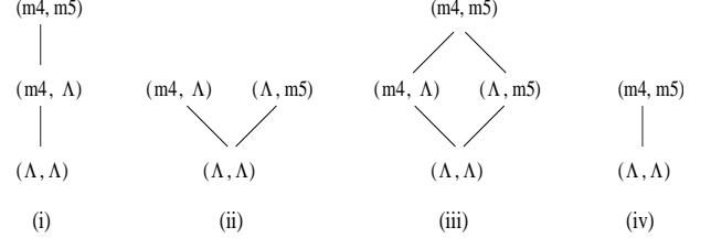
Fig. 3. Order structure and dependencies between agents' moves
