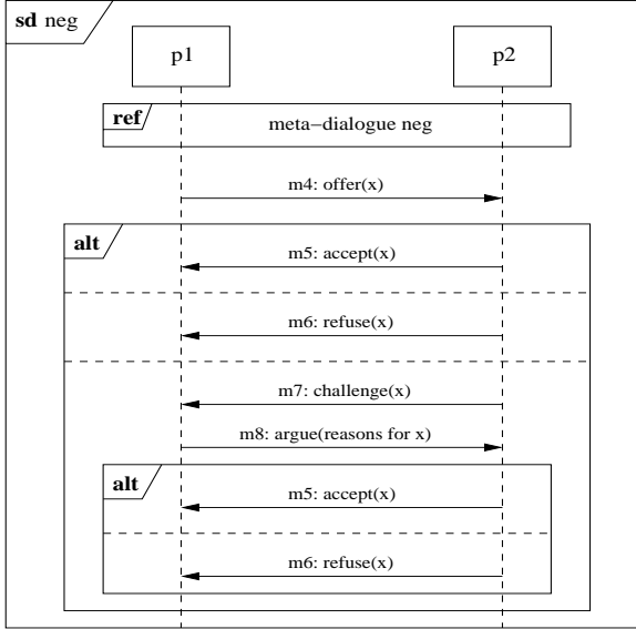
Fig. 4. UML sequence diagram for the negotiation dialogue protocol
