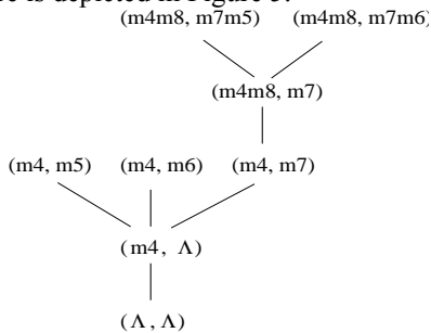
Fig. 5. Order structure of a negotiation dialogue language
