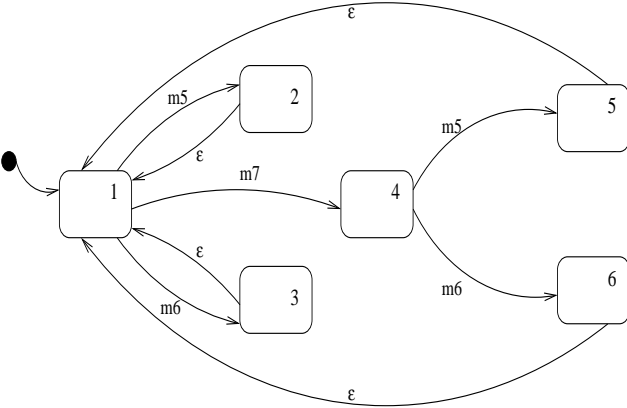
Fig. 2. UML PSM for agent a2 in a negotiation dialogue
