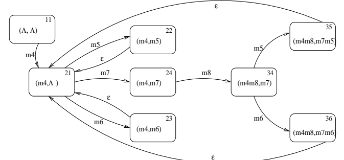
Fig. 6. UML state diagram for available moves in a negotiation dialogue
