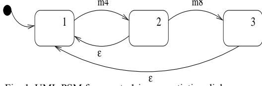
Fig. 1. UML PSM for agent a1 in a negotiation dialogue
