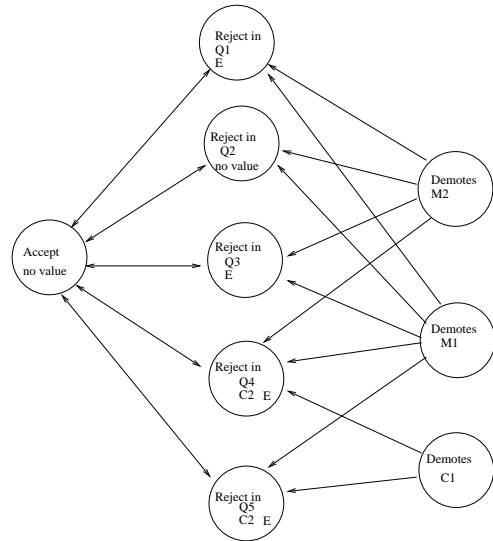
Figure 2: VAF for acceptance or rejection
