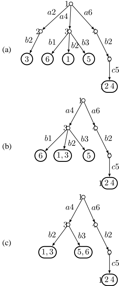
Fig. 6. Updates of the signature trie of Figure 5. The initial trie is given in Figure 5. (a) After updating arcs labeled by b . (b) After updating arcs labeled by a . This is the result of merging 2 and 4. (c) Result of merging 1 and 3: update of the arcs labeled by d . The merging of states 5 and 6 does not change the trie.
