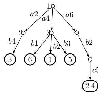
Fig. 5. The initial signature trie of the automaton of Figure 3. It is rooted at the node 1. Only one leaf contains more than one state, namely states 2, 4. They have the same signature a6b2c5 .
